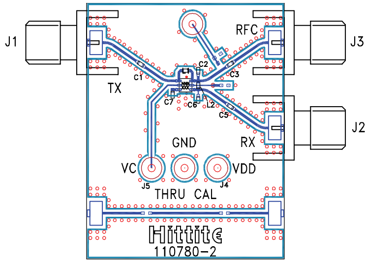
Figure 26. Evaluation Printed Circuit Board (PCB)
