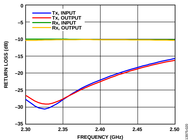
Figure 19. Return Loss vs. Frequency
