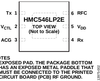
Figure 2. Pin Configuration
