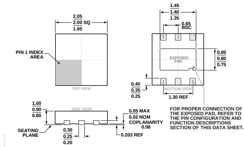
Figure 27. 6-Lead Lead Frame Chip Scale Package [LFCSP] 2 mm × 2mm Body and 0.90 mm Package Height (CP-6-10) Dimensions shown in millimeters
