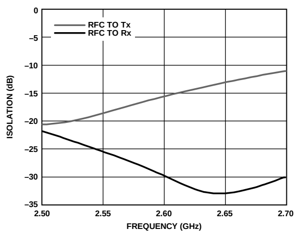
Figure 21. Isolation vs. Frequency
