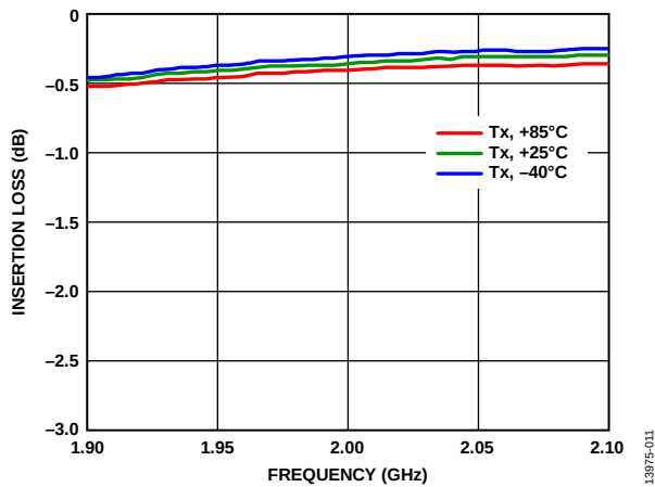
Figure 10. Tx to RFC Insertion Loss vs. Frequency over Temperature
