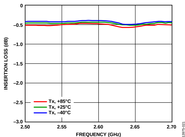
Figure 20. Tx to RFC Insertion Loss vs. Frequency over Temperature
